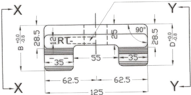
TOP PLAN
