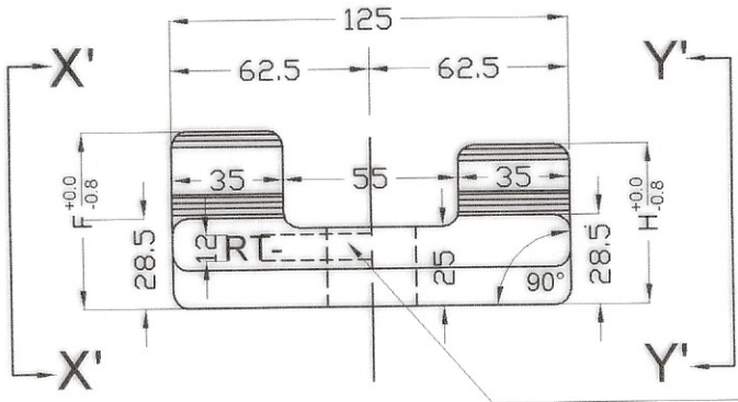
TOP PLAN
